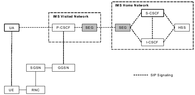
Figure 2. IMS authentication architecture
