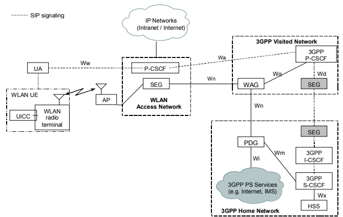
Figure 3. Proposed authentication solution architecture
