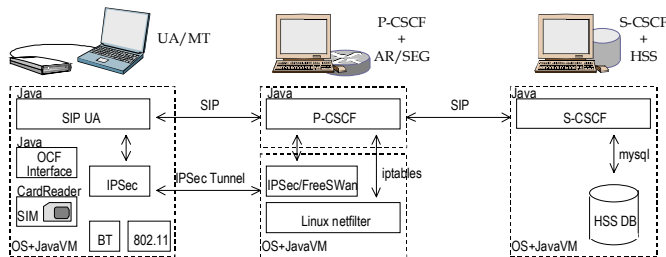
Figure 6. Implementation architecture
