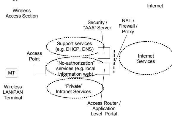
Figure 1. Exemplary Wireless LAN/PAN access architecture
