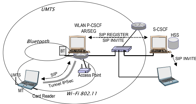
Figure 5. Implementation testbed layout
